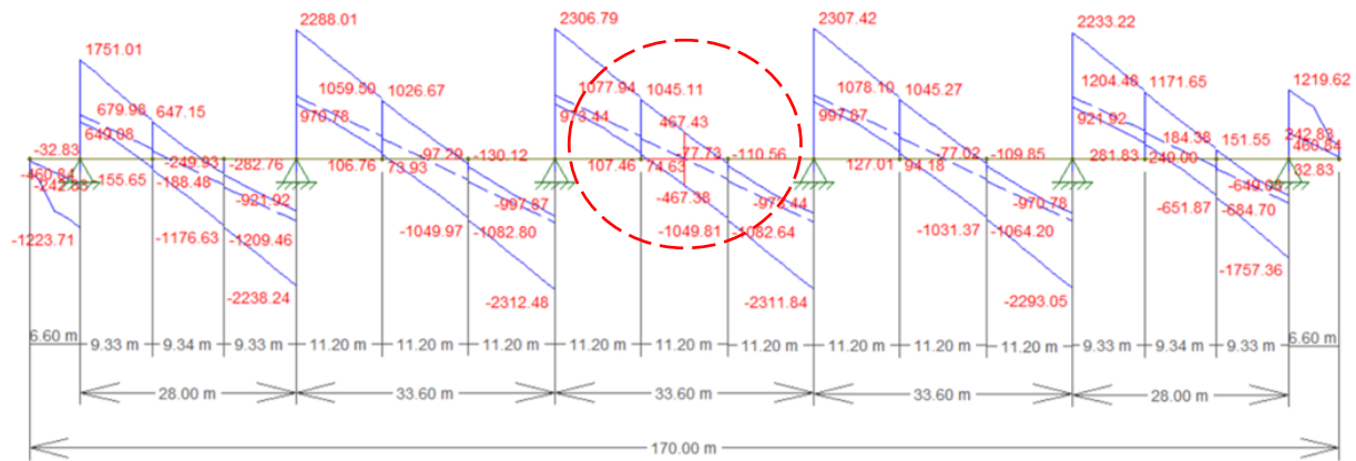
Figure 3. Shearing envelope with TB-450 increased by WCV (ABNT NBR 7188, 2013).
