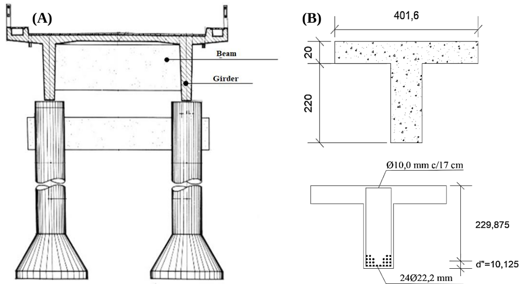
Figure 1. (A) Bridge's cross section over the Chapecó River; (B) Cross section, in centimeters, of the investigated section of the girder (Adapted from the Departamento de Estradas e Rodagem Santa Catarina, 1987).
