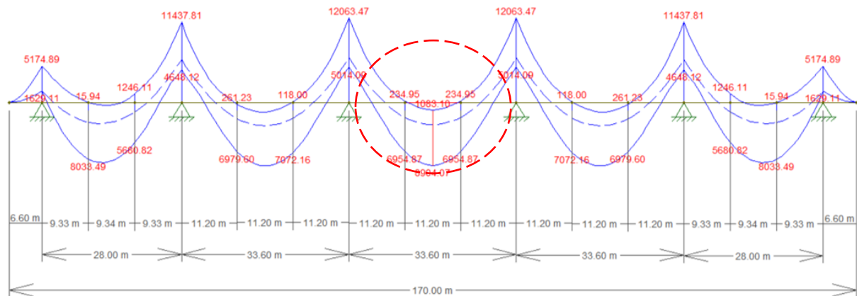
Figure 4. Bending moment envelope with TB-450 increased by WCV (ABNT NBR 7188, 2013).
