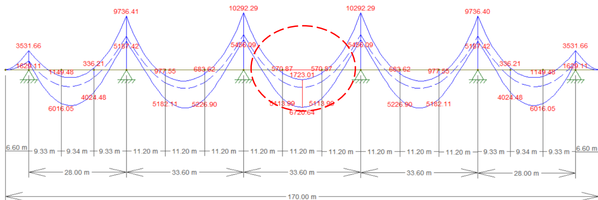
Figure 2. Envelopment of efforts due to the 300 Brazilian Load Model and \phi = 1.23 .
