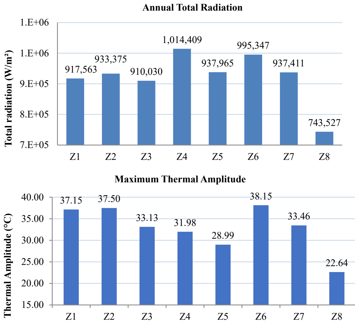
Figure 2. Total accumulated radiation and maximum thermal amplitude in the simulation year.
