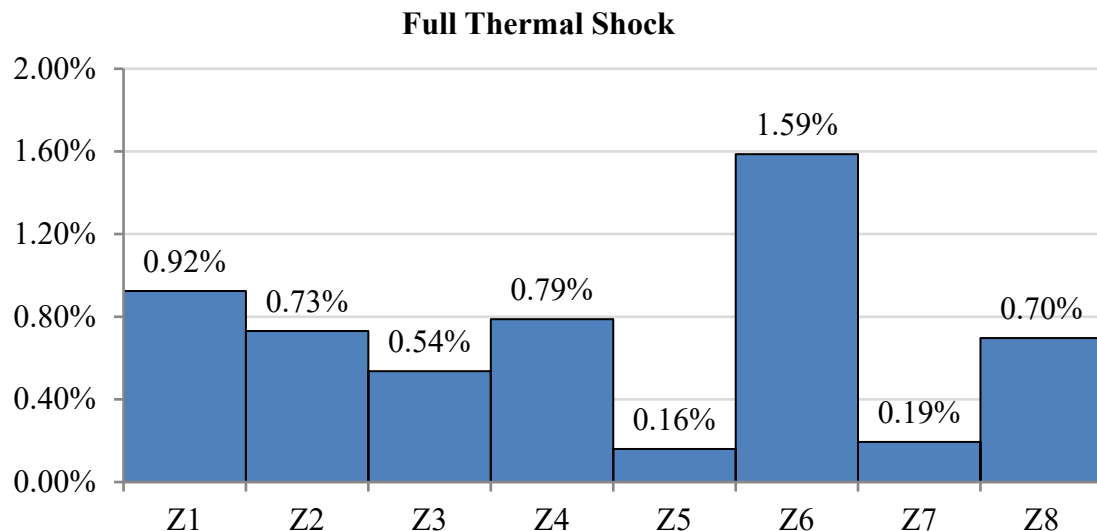
Figure 4. Frequency of occurrence of full thermal shock during one year.
