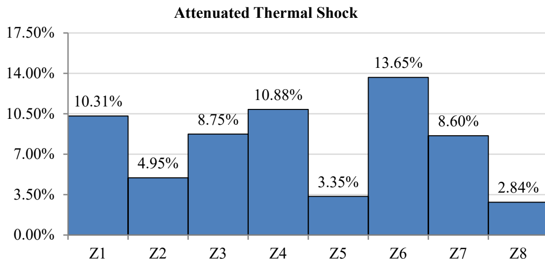
Figure 5. Frequency of attenuated thermal shock observed in one simulation year.
