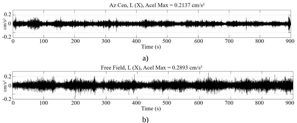
Figure 14. Ambient vibration (VA) signals located at the geometric center of the roof (Az Cen) L(X) and free field (CL) L(X); a) Az Cen L(X); b) CL. Where L=longitudinal, Az = roof.
