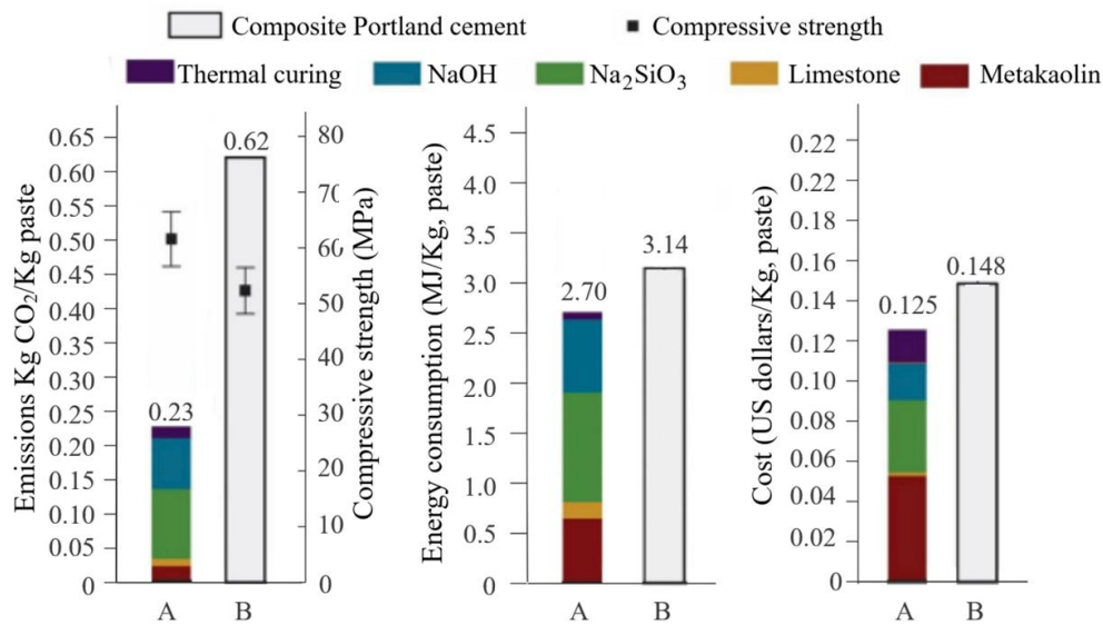
Figure 6. Comparison of CO 2 emissions, energy consumption, and cost between: A - AAC (60% limestone, 40% metakaolin); and B - composite PC. Adapted from (Pérez-Cortés & Escalante-García, 2020a)
