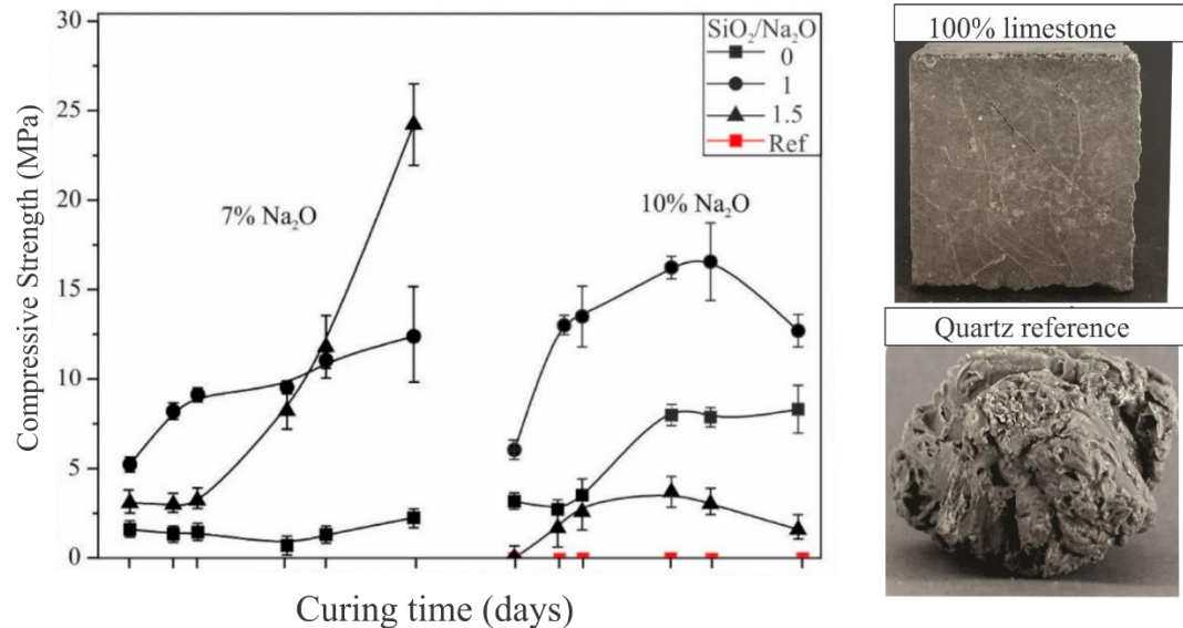
Figure 4. Compressive strength and photographs of alkali-activated limestone and quartz (red line) hardened cements. Adapted from (Ortega-Zavala et al., 2019).
