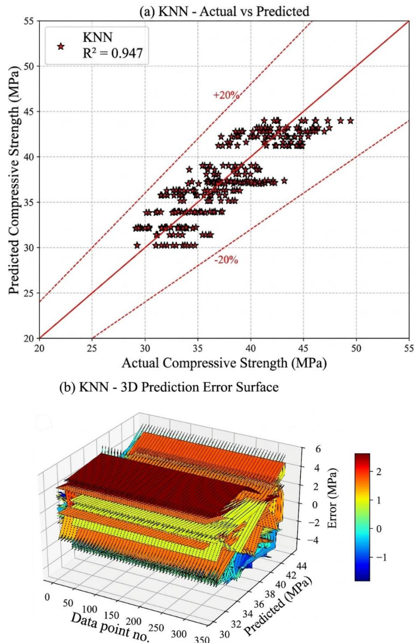
Figure 12. K-Nearest Neighbors model performance for predicting 28-day compressive strength of concrete. (a) Scatter plot of actual versus predicted compressive strength, (b) 3D surface plot depicting the distribution of prediction errors across all data points.
